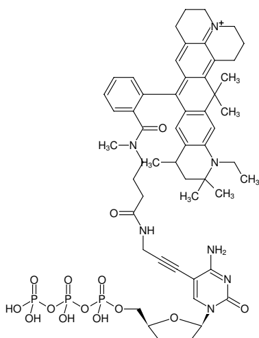
Structural formula of 5-Propargylamino-ddCTP-ATTO-647N
