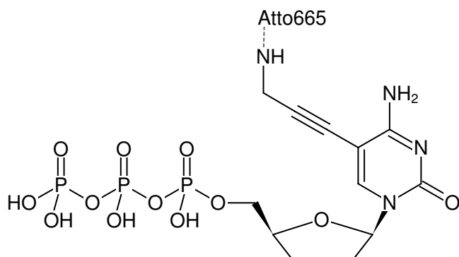
Structural formula of 5-Propargylamino-ddCTP-ATTO-665
