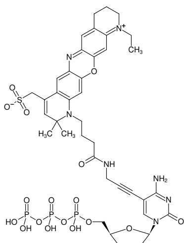
Structural formula of 5-Propargylamino-ddCTP-ATTO-680
