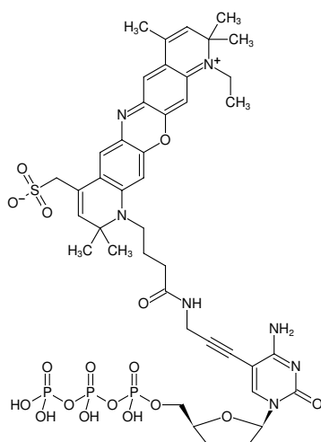
Structural formula of 5-Propargylamino-ddCTP-ATTO-700
