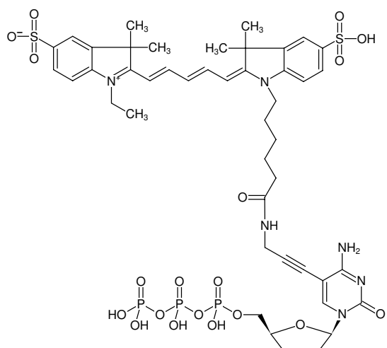
Structural formula of 5-Propargylamino-ddCTP-Cy5
