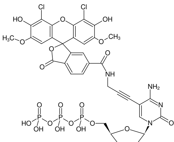
Structural formula of 5-Propargylamino-ddCTP-6-JOE
