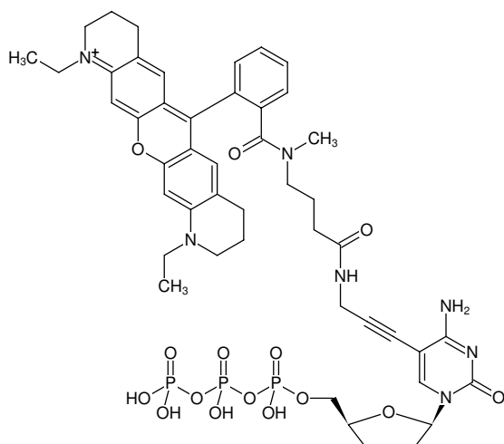
Structural formula of 5-Propargylamino-ddCTP-ATTO-Rho11
