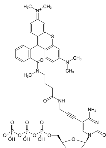
Structural formula of 5-Propargylamino-ddCTP-ATTO-Thio12
