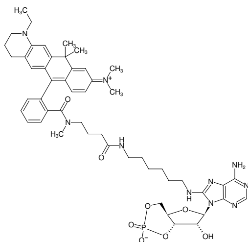
Structural formula of 8-(6-Aminoethyl)-amino-cAMP-ATTO-633
