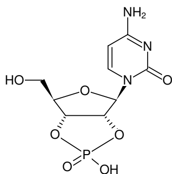
Structural formula of Cytidine-2',3'-cyclic monophosphate
