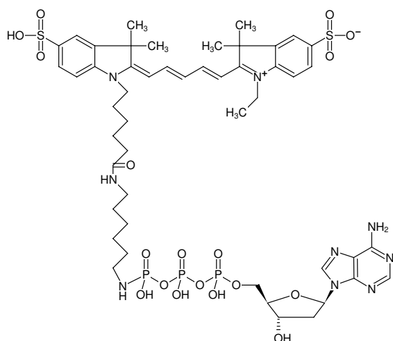
Structural formula of \gamma -[(6-Aminohexyl)-imido]-dATP-Cy5
