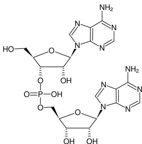
Structural formula of ApA
