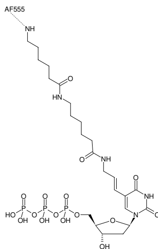
Structural formula of AF555 NT Labeling Kit
