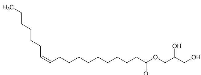
Structural formula of Monovaccenin
